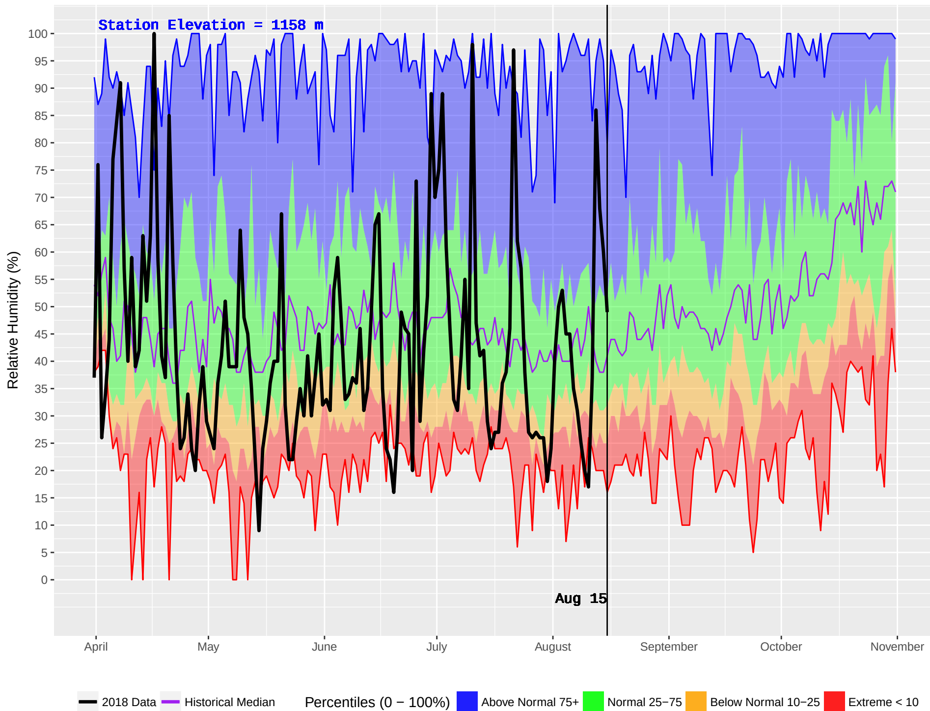
LONE BUTTE (218) : Historical (1987–2016) and Current (2018) Daily Relative Humidity
