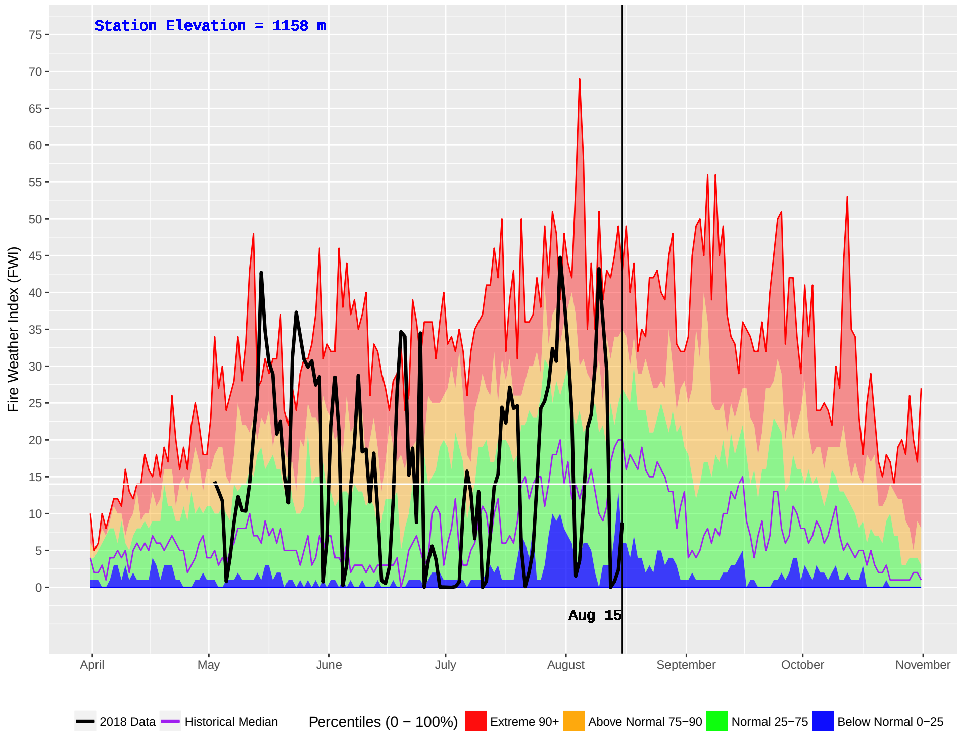
LONE BUTTE (218) : Historical (1987–2016) and Current (2018) Daily Fire Weather Index (FWI)
