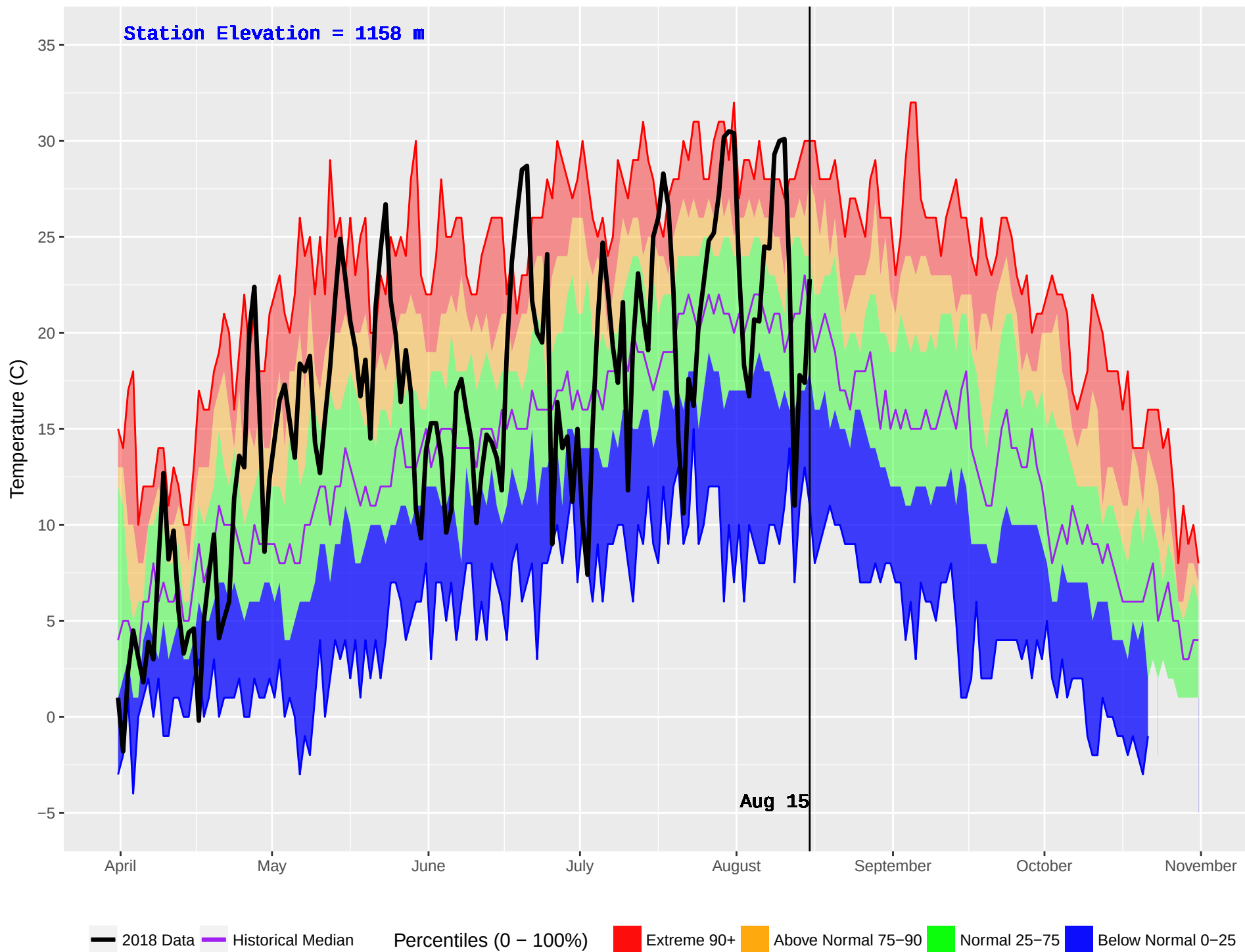
LONE BUTTE (218) : Historical (1987–2016) and Current (2018) Daily Temperature
