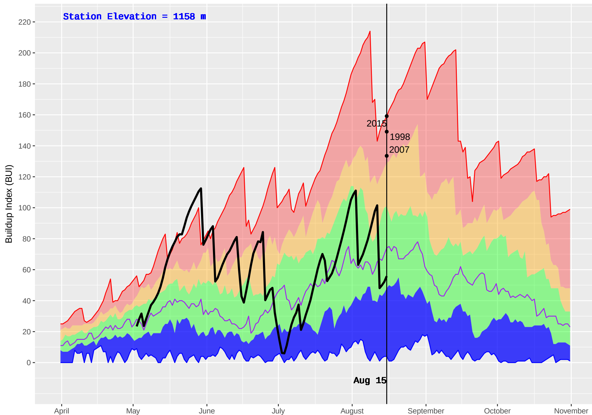
LONE BUTTE (218) : Historical (1987–2016) and Current (2018) Daily Buildup Index (BUI)
